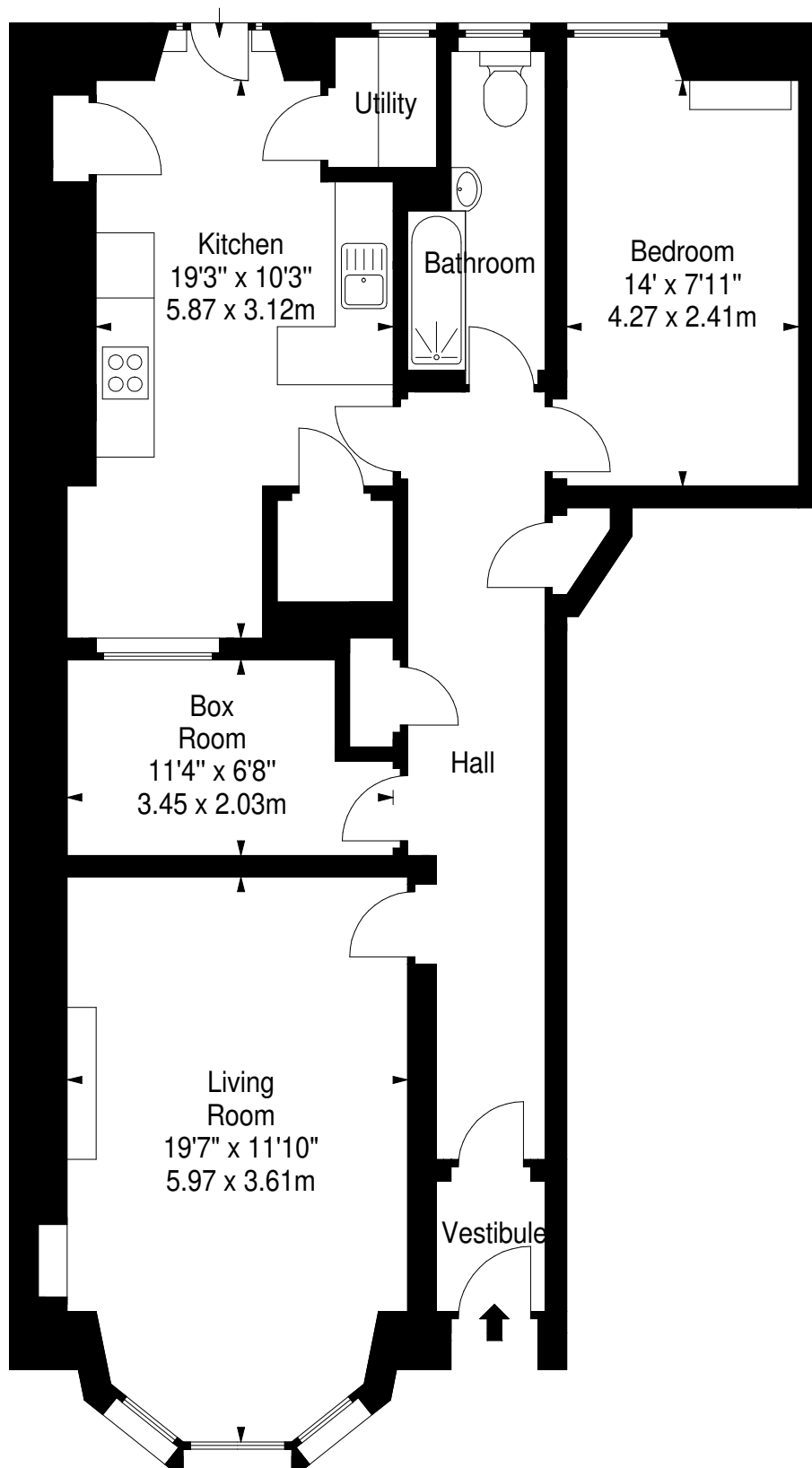
Ground Floor
