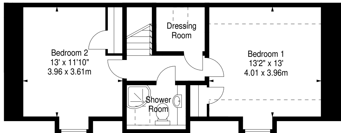
Second Floor
