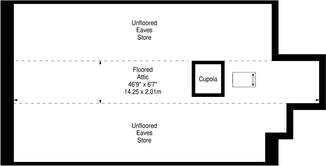
Attic
