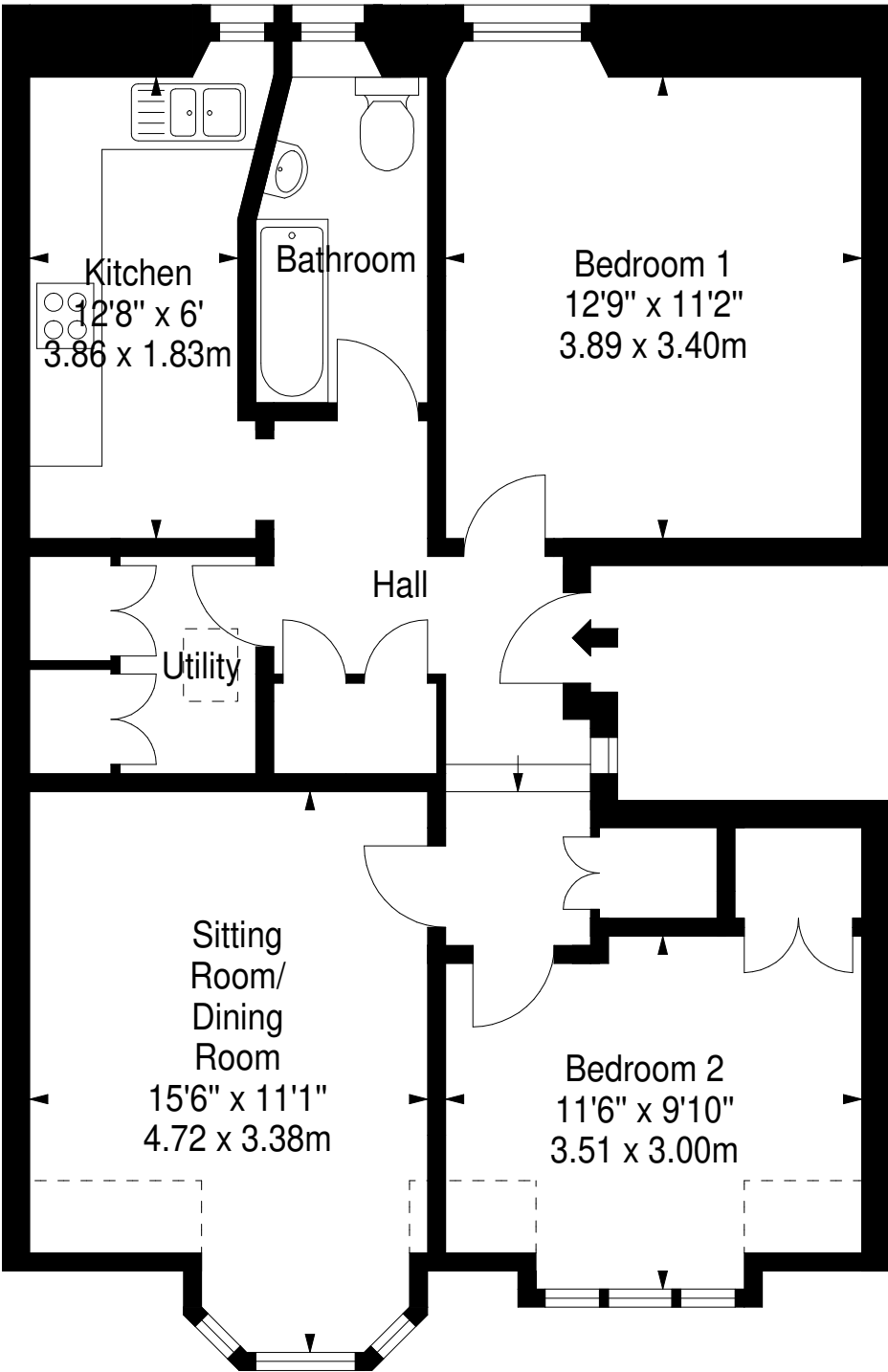
Second Floor
