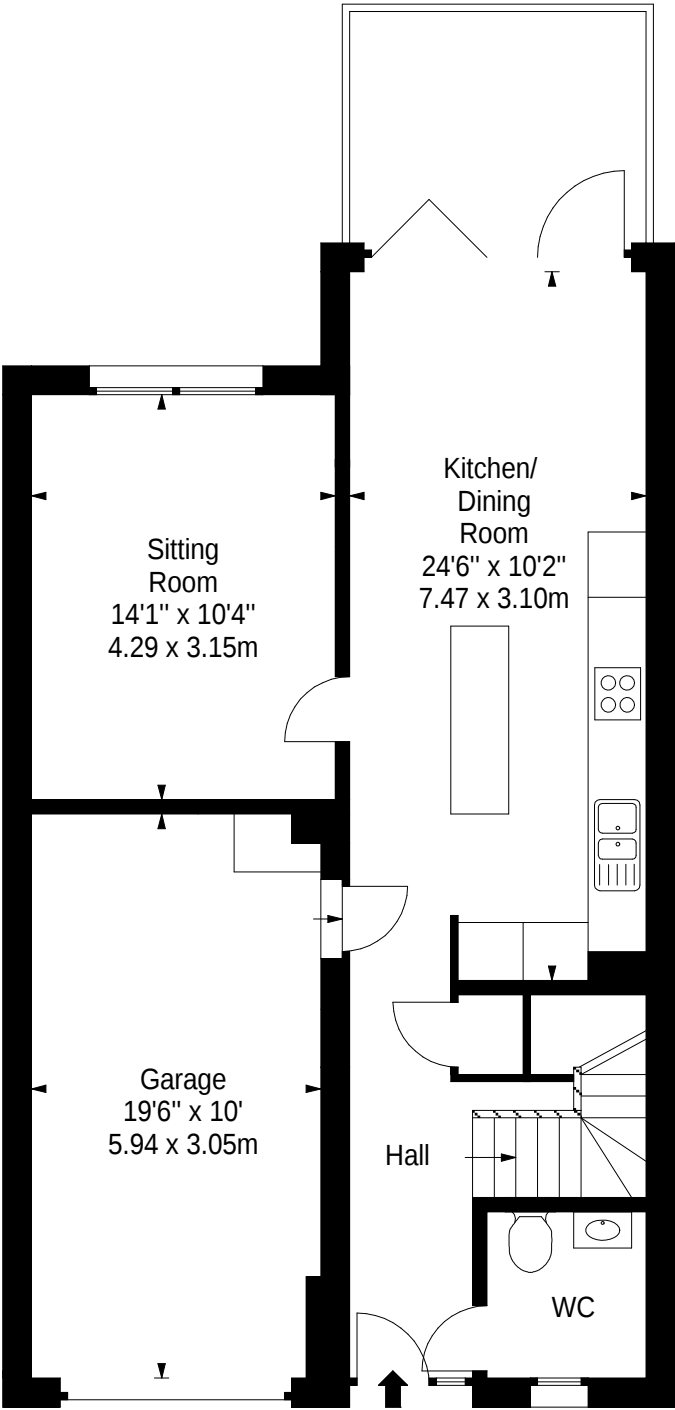
Ground Floor
