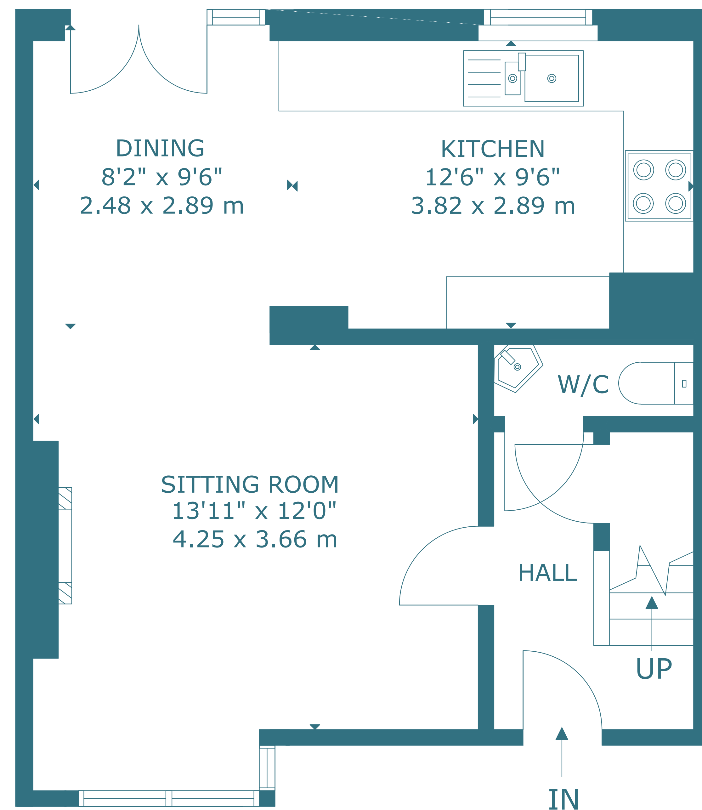
GROUND FLOOR
