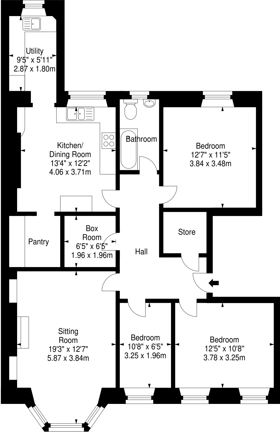
First Floor
